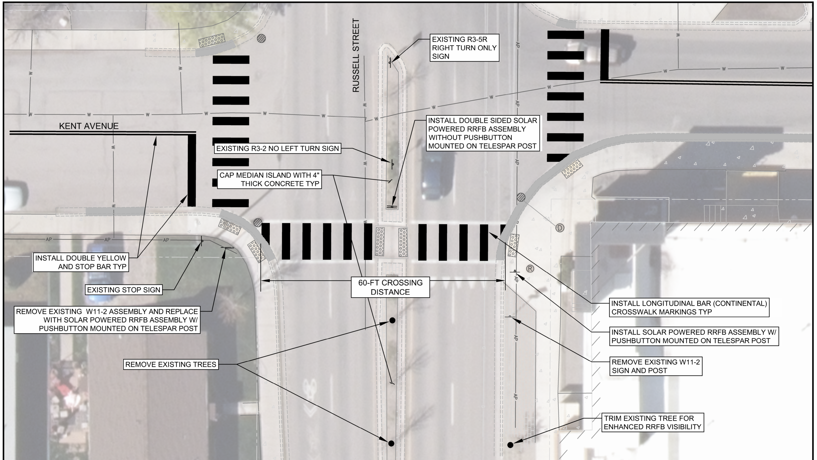
RUSSELL STREET & KENT AVENUE CROSSWALK PROPOSED RRFB ENHANCEMENT CONCEPTUAL PLAN
